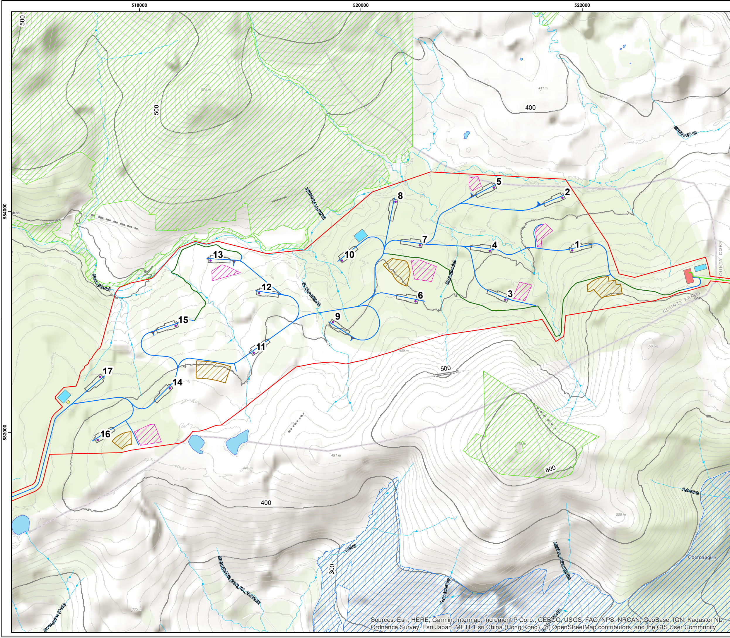
Figure10-1b 10m Contour Map
